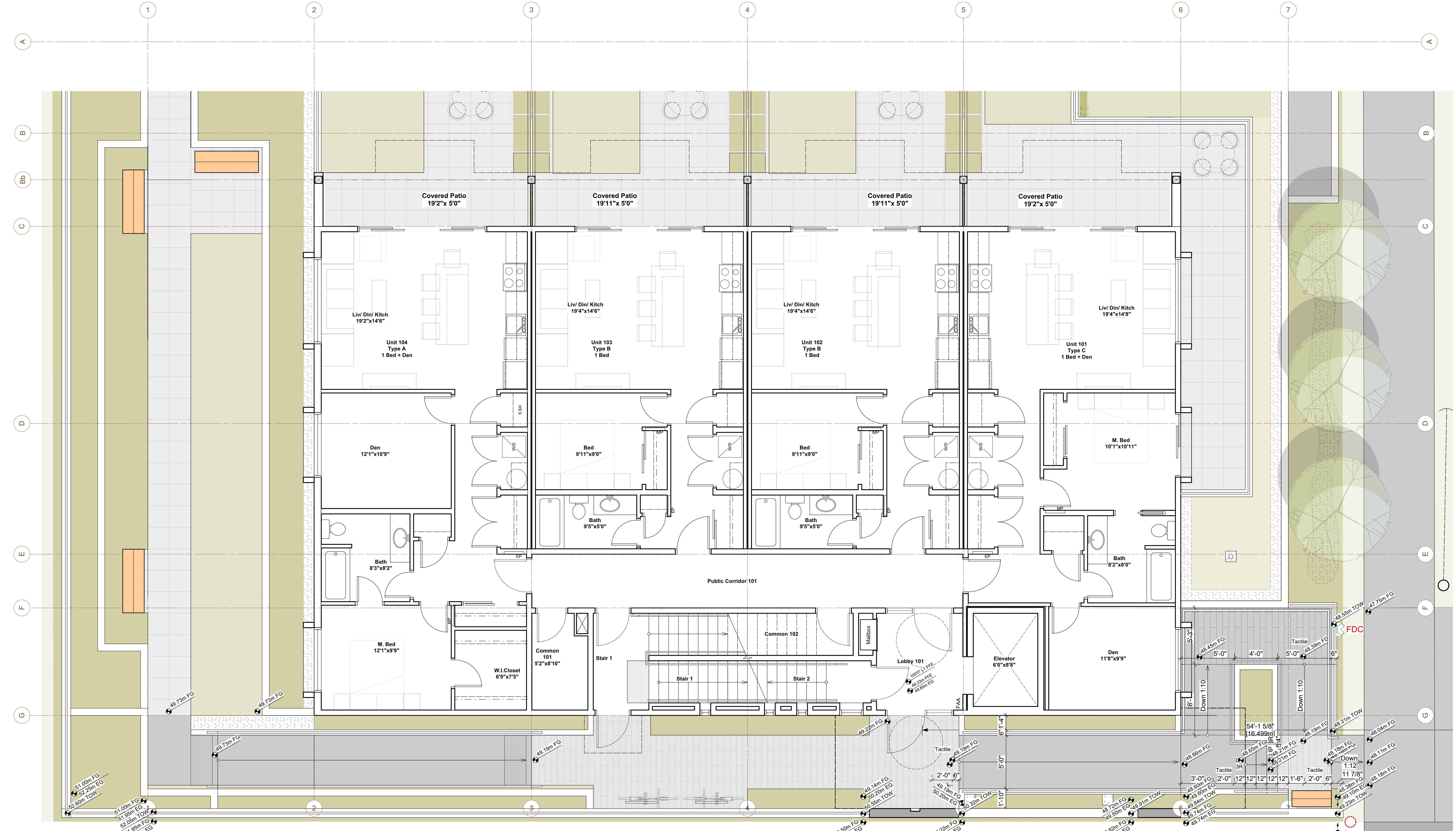
10 L1 FLOOR PLAN Scale: 1/4" = 1'-0"
